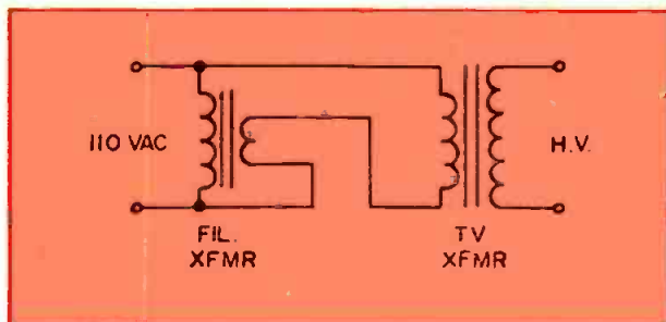
Fig. 6 Buck/boost transformer for adjusting voltage. Polarity of transformer determines increase or decrease.
