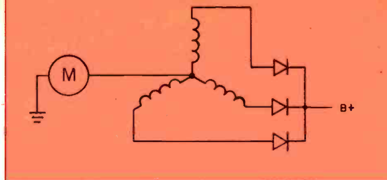
Fig. 7 Emergency 3-phase half-wave rectifier. Voltage will be approximately 50% of normal.
