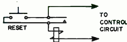
Fig. 4 Latching relay for troubleshooting intermittents.
