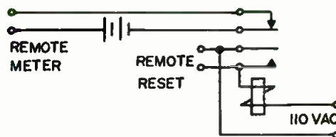
Fig. 5 Power failure detector for remote transmitter sites.
